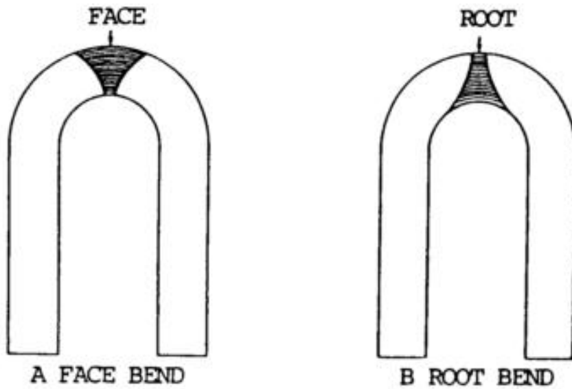
Figure 13-2. Guided bend test specimens.
